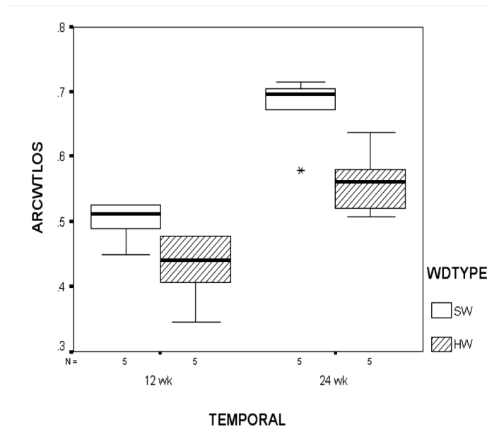
Figure 1. Weight loss variation in Parashorea sapwood and heartwood wood blocks after 12 and 24 weeks exposure to the test fungus. The dependent variable of percent weight loss was arcsine (square root (proportion of weight loss)) transformed. (n replicates= 5)
